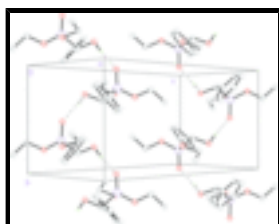
Fig. 3. Part of the crystal structure of I , showing chiral helical chains aligned in an antiparallel fashion. The H atoms not involved in H-bonds are omitted for clarity.
