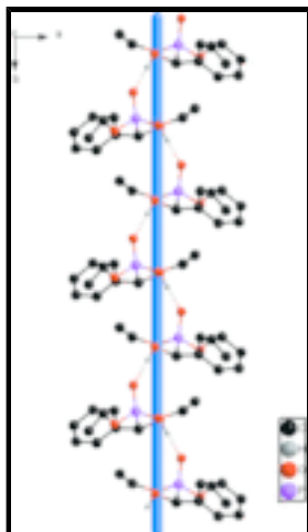
Fig. 2. The chiral helical chain constructed by O—H···O H-bonds.
