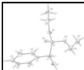
Fig. 1. A molecular structure of I with the atom numbering scheme. Displacement ellipsoids are drawn at 30% probability level. Only major part of disordered moiety are presented. The H atoms are drawn as a small spheres of arbitrary radius.
